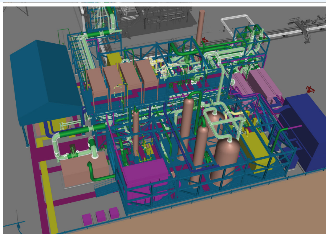
Photo: the pilot plant project at Esso Nederland BV Rotterdam Manufacturing Complex
